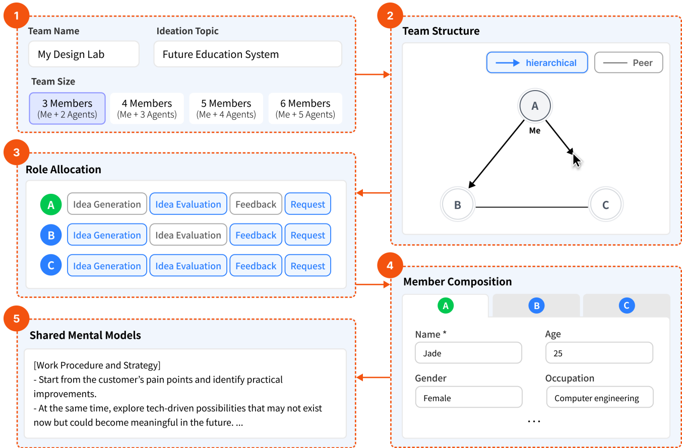
Figure 2: Simplified Team Formation Interface of CRAFTeAM. (1) The user sets the team name and ideation topic and chooses the team size. (2) The user configures a networked team structure by linking members as hierarchical or peer. (3) The user assigns roles to each member—Idea Generation, Idea Evaluation, Feedback, and Request. (4) The user creates member personas in a resume-like form aligned with roles. (5) The user establishes the team’s shared mental models.
