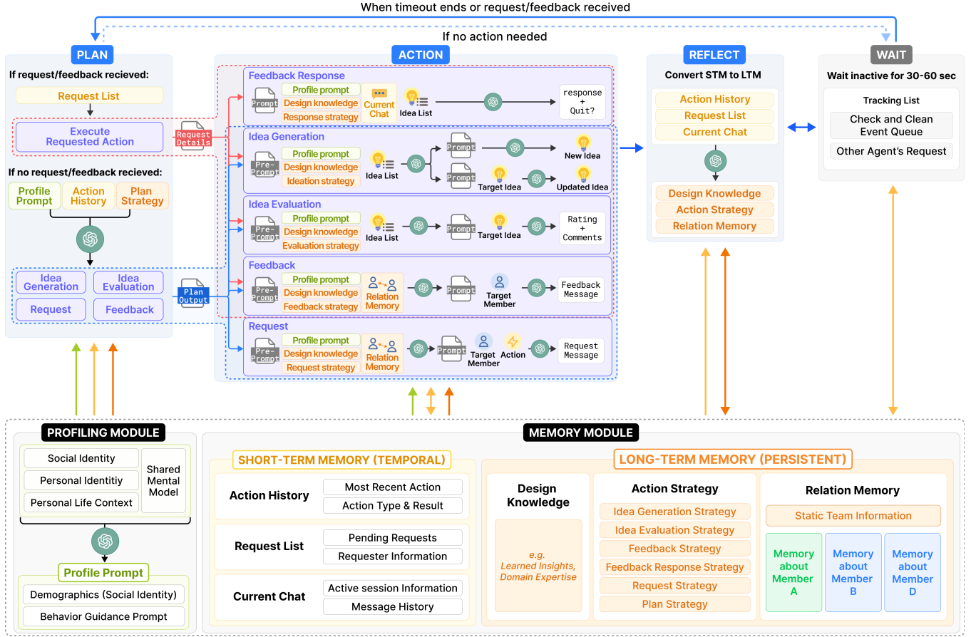
Figure 8: Agent architecture of CRAFTTEAM. Agents iterate through Plan → Act → Reflect → Wait states. During the Act state, role-permitted action pipelines are executed. Agent operations are governed by two modules: a Profiling module and a Memory module that separates short-term memory from long-term memory.
